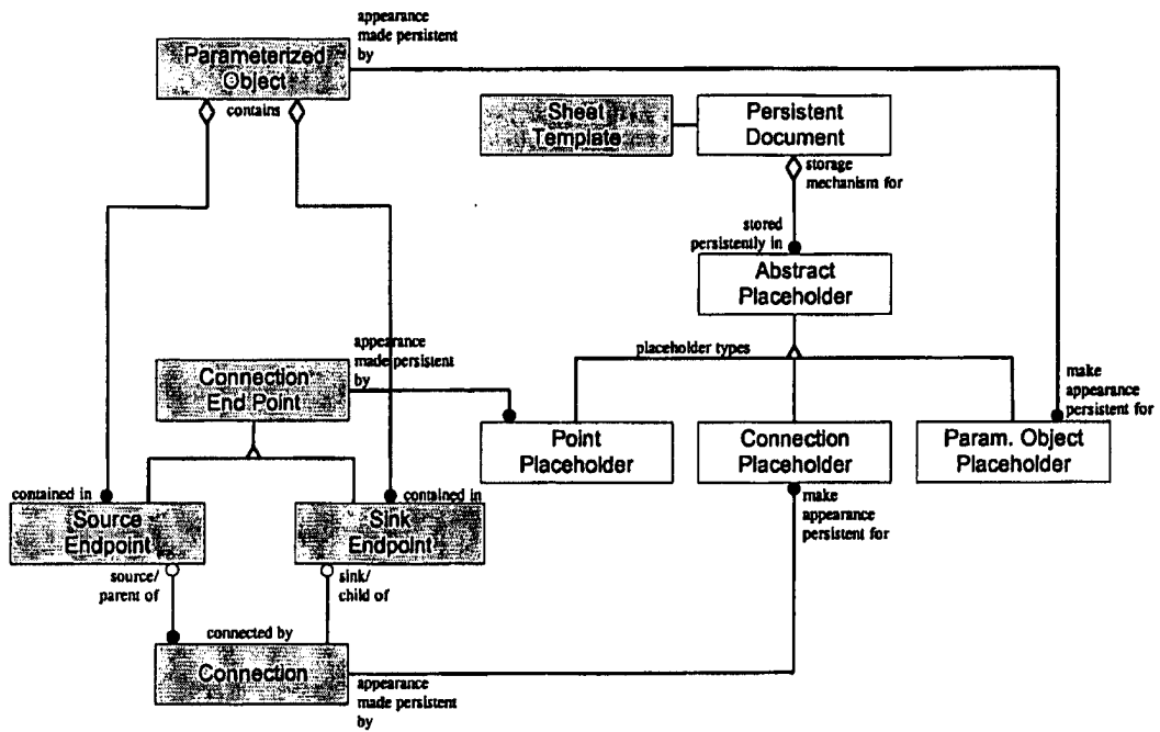
Figure 29A - Placeholders Object Model
